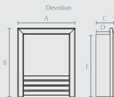
A) Width 510mm B) Height 605mm C) Depth 174mm D) Inset 140mm E) Rear Height 555mm
