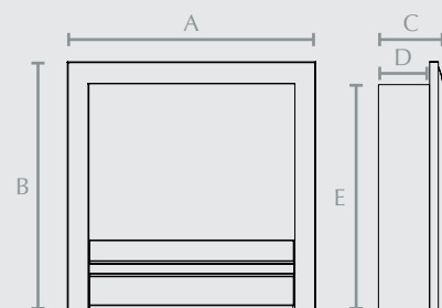
A) Width 611mm B) Height 611mm C) Depth 170mm D) Inset 140mm E) Rear Height 565mm
