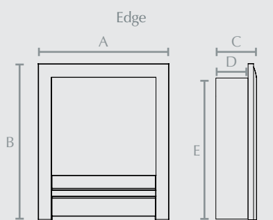
A) Width 511mm B) Height 611mm C) Depth 174mm D) Inset 140mm E) Rear Height 555mm
