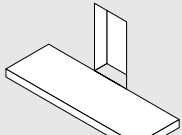
Pre-cast/ Class 1 flue opening
