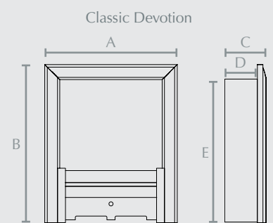
A) Width 510mm B) Height 605mm C) Depth 174mm D) Inset 140mm E) Rear Height 555mm
